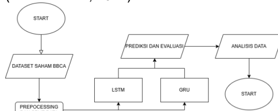
Gambar 1. Diagram Alur ( Flowchart ) Penelitian
